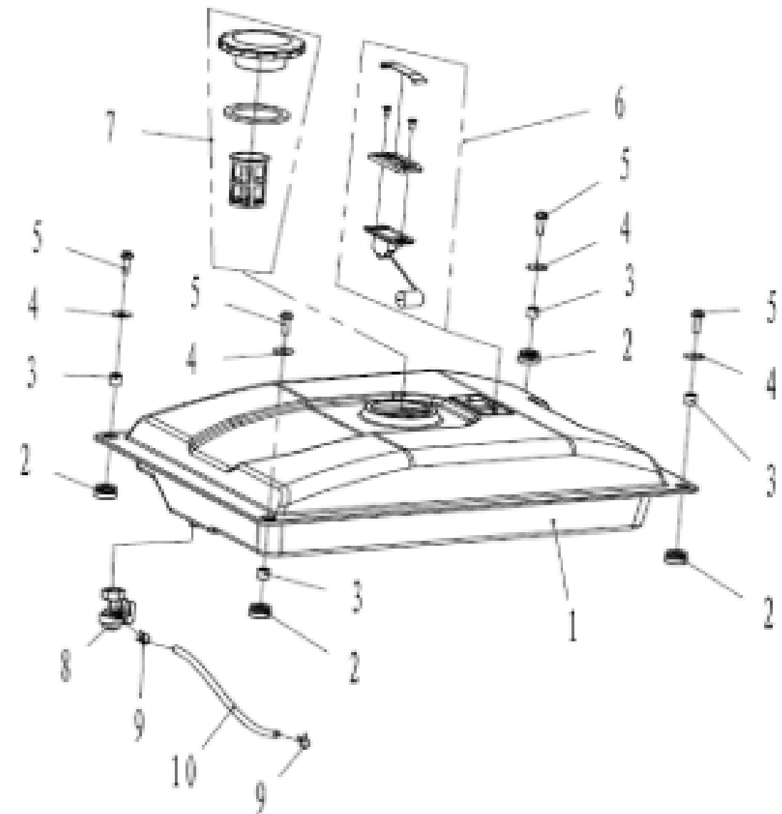
油箱组件 Fuel tank assembly
